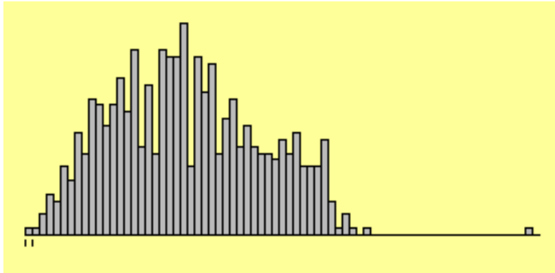
Figure 2 A histogram of the age distribution from figure 1.
